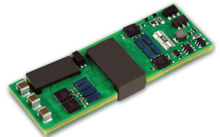
1/8 power brick featuring the EPC2001 eGaN FET and LM5113 GaN FET driver.
