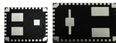
PMP8372 reference design.
