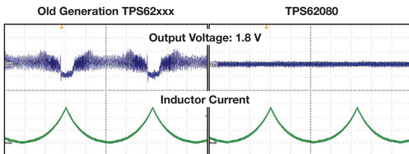
Seamless transition between PWM and Power Save mode with V IN = 3.6 V and a 0- to 500-mA triangle load sweep.
